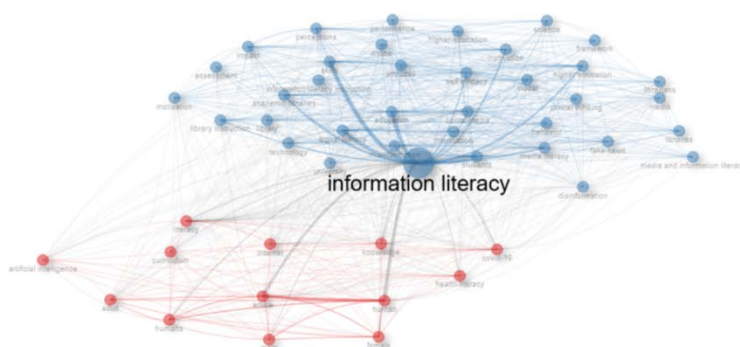
Fig. 6. Co-occurrence network
